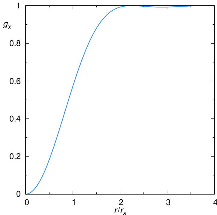
Figure 2.1: Exchange hole g_x(\vec{r}) in the homogeneous electron gas.
