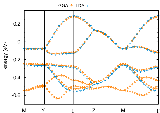
Fig. 3. Comparison of low energy band structure between different exchange and correlation potentials for \kappa -(BEDT-TTF) 2 X with X = Cu 2 (CN) 3 . The FPLO basis set was used. For GGA, two Cu 3d bands are entangled with the bonding bands of the BEDT-TTF dimer molecules; for LDA, they are clearly separate (starting below about -0.6 eV) and therefore not shown.
