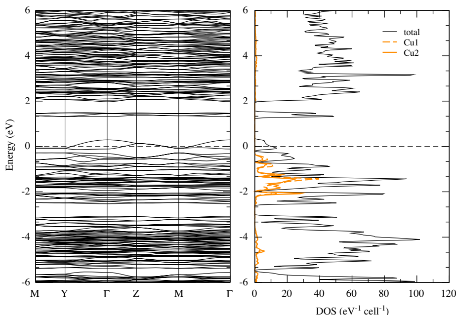
Fig. 2. Band structure and density of states of \kappa -(BEDT-TTF) 2 X with X = Cu 2 (CN) 3 , calculated with FPLAPW. The contribution of Cu to the DOS is highlighted. The Cu 3d states are fully occupied, indicating that Cu is in a nonmagnetic Cu + oxidation state.
