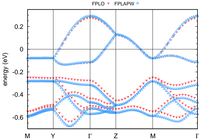
Fig. 4. Comparison of low energy band structure between FPLAPW and FPLO basis sets for \kappa -(BEDT-TTF) 2 X with X=Cu 2 (CN) 3 . The GGA exchange and correlation potential was used.
