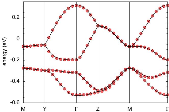
Fig. 5. Low energy bandstructure of \kappa -(BEDT-TTF) 2 X with X=Cu(SCN) 2 (symbols) and tight binding fit (lines). Note the lifting of the degeneracy at the Z point.
