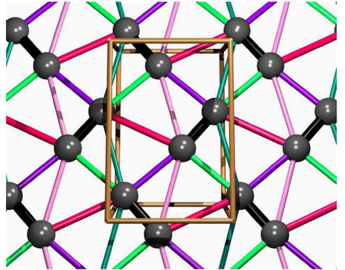
Fig. 6. Lattice of BEDT-TTF molecules (gray spheres) for \kappa -(BEDT-TTF) 2 X with X=Cu(SCN) 2 . Dimer bonds ( t_1 ) are shown in black, t_4 \equiv t' in red. t has to be calculated from an average over t_2 (light green), t_3 (purple), t_5 (dark green) and t_6 (pink). The view is along the a direction, and the unit cell is marked. (For interpretation of the references to color in this figure legend, the reader is referred to the web version of this article.)
