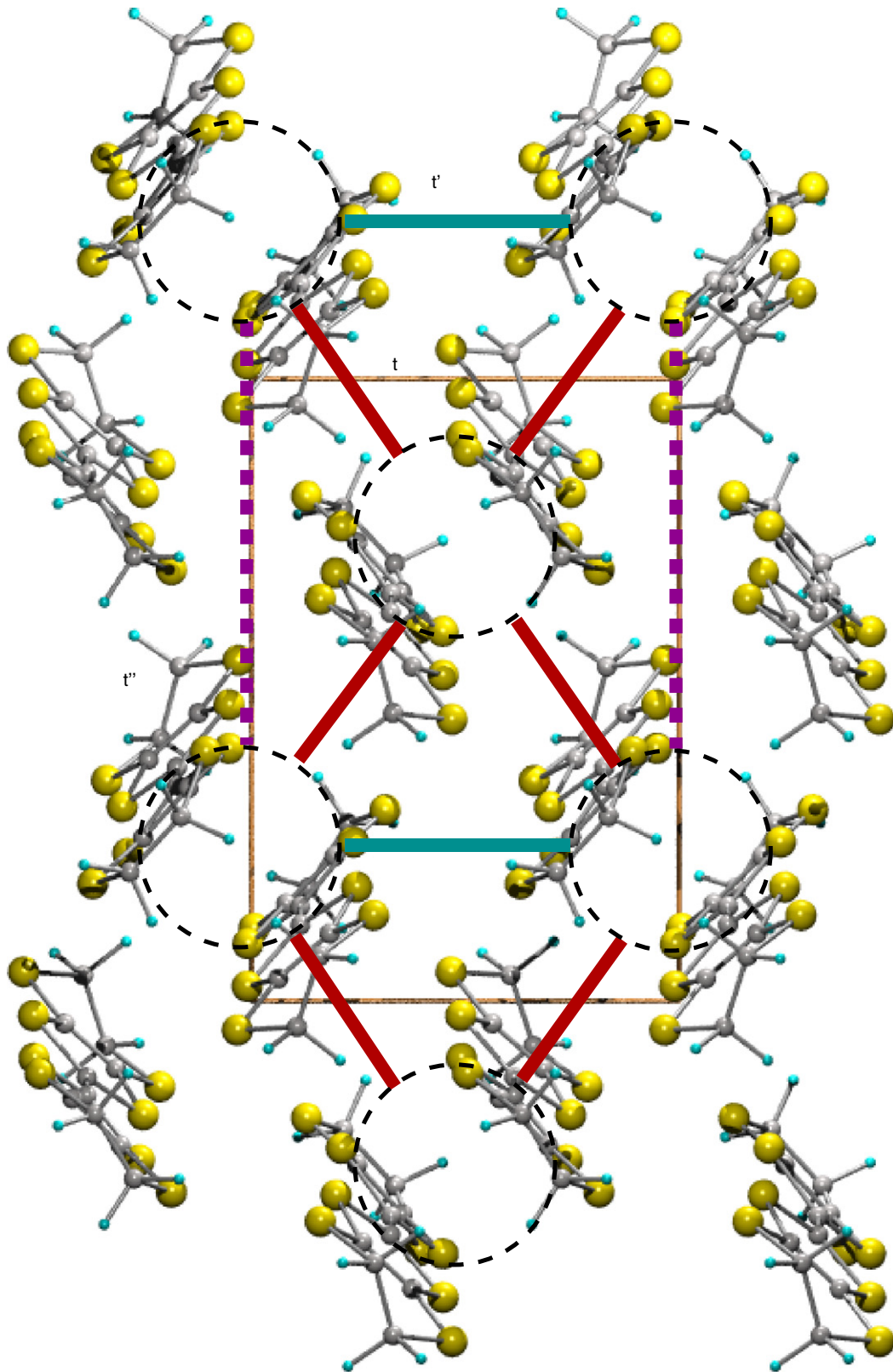
Fig. 1. Structure of the \kappa BEDT-TTF arrangement for the example of \kappa -(BEDT – TTF) 2 X with X = Cu 2 (CN) 3 . t and t' form a frustrated triangular lattice.
