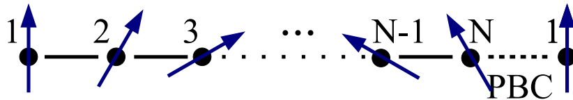
Figure 6.2: Spin spiral that is commensurate with the size of the system due to the periodic boundary condition (PBC).
